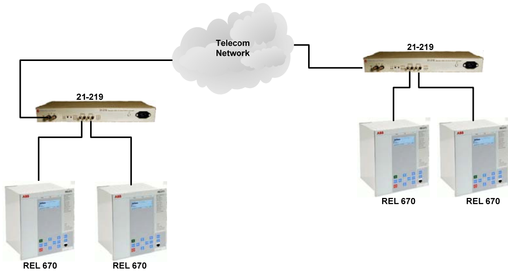
Dual IEEE C37.94 link via Telecom network.
